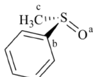
(S)-(methanesulfinyl)benzene (PIN)
