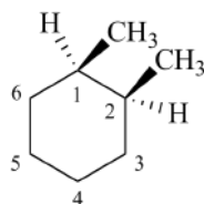
(1R,2S)-1,2-dimethylcyclohexane (PIN)
