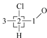
simplified digraph
